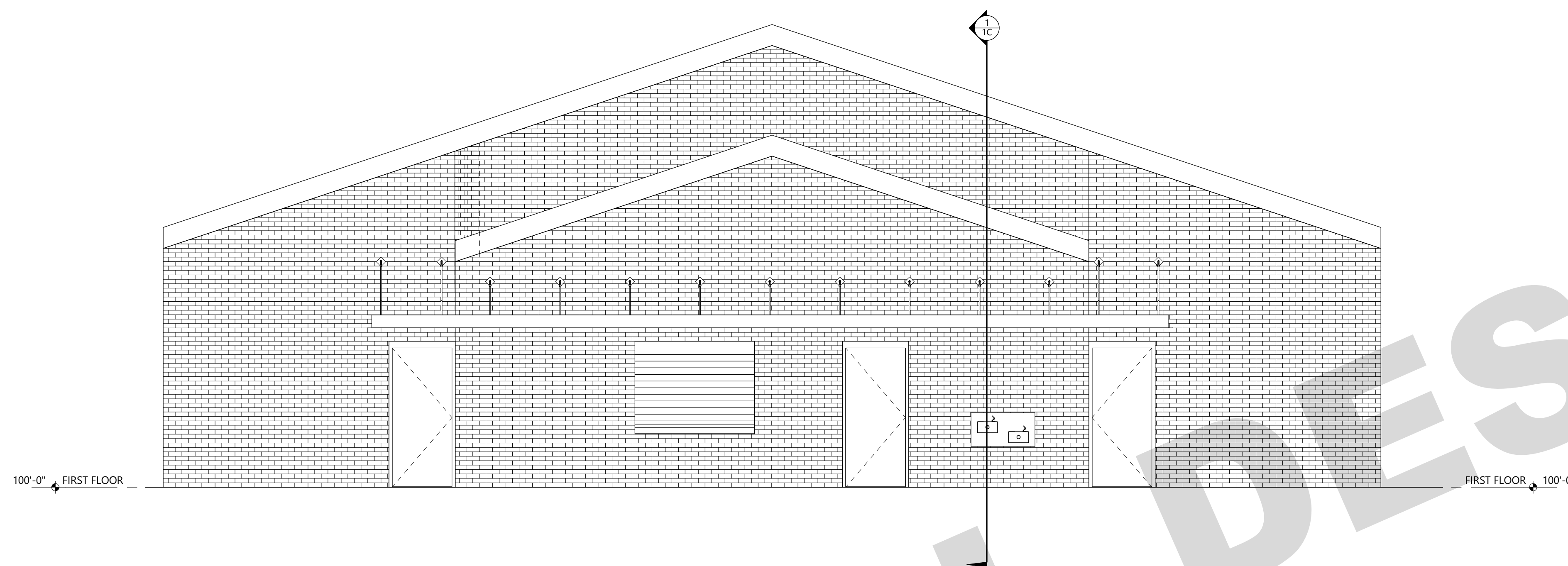
1 Building Elevation 1/4" = 1'-0"
