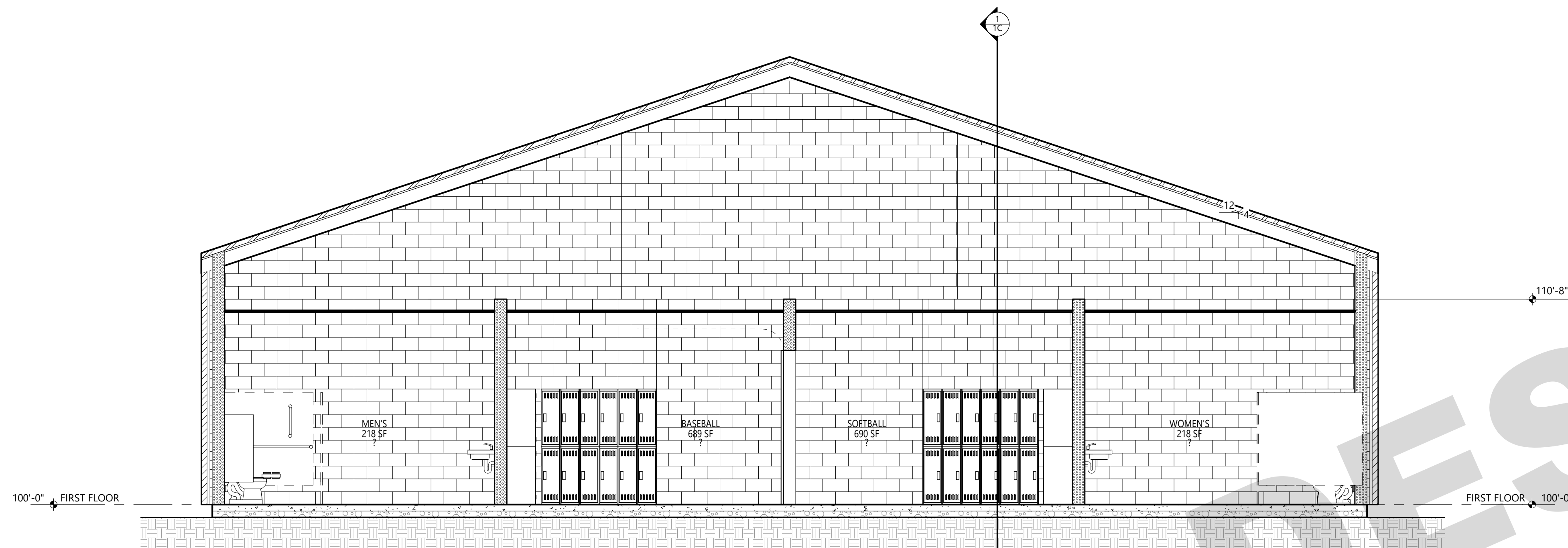
2 Building Section 1/4" = 1'-0"
